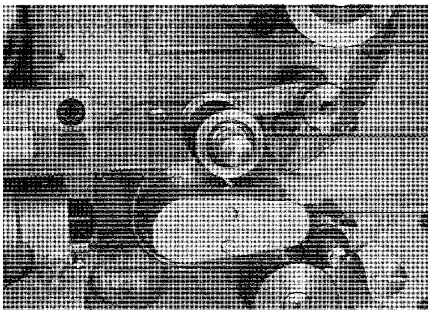
Fig. 5-5: Soundhead Threading
