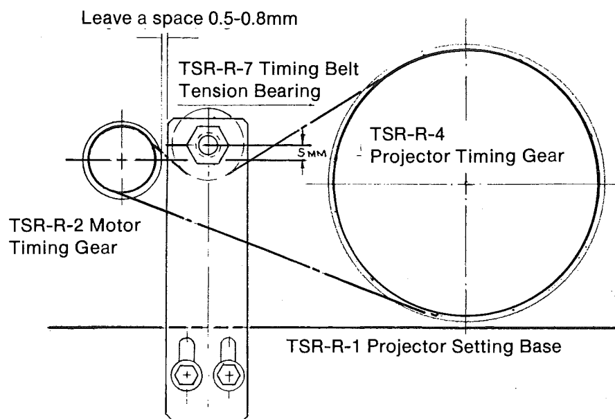
Fig. 6-4: Timing Belt Tension Bearing Setting Point
