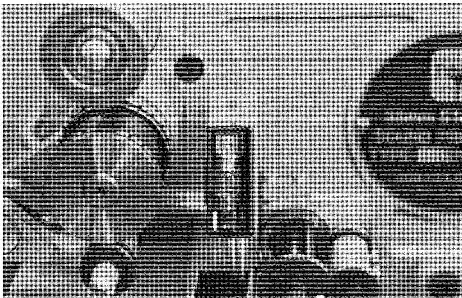
Fig. 4-1: Framing Lamp Assembly (Open)
