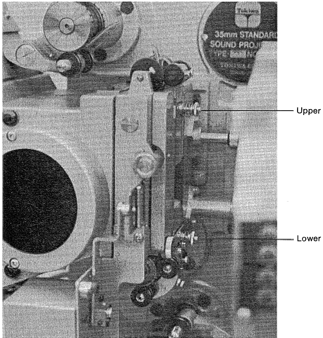
Fig. 5-6: Gate Pad Adjustment Collars
