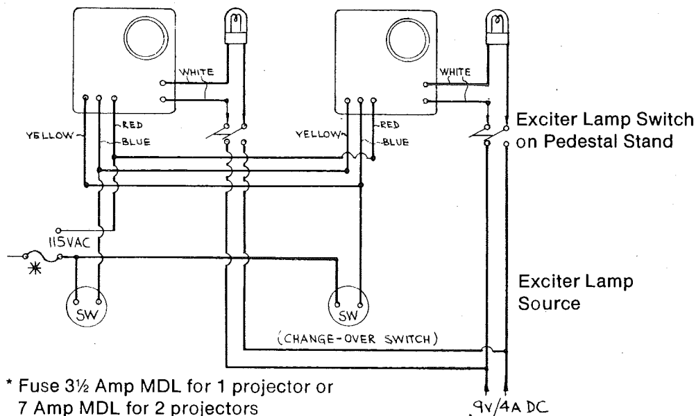
4-2: Connection Diagram for Changeover Switch
