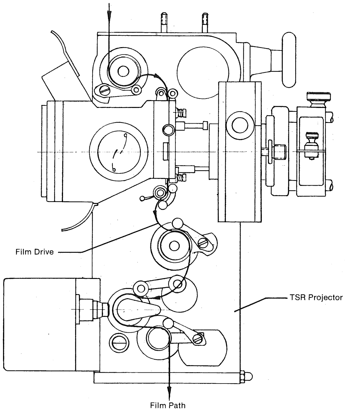
Fig. 5-3: Threading Diagram
