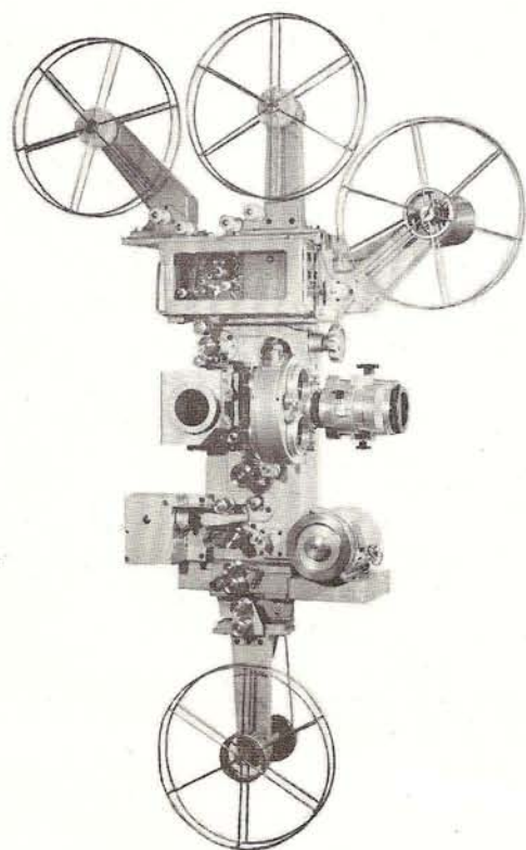
↑ ■ TOKIWA TSR-3000 PROJECTION MECHANISM WITH 3000FT MAGAZINE
