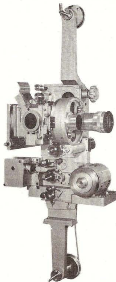
↑ ■ TOKIWA TSR-3000 PROJECTION MECHANISM WITH 6000FT REEL ARM
