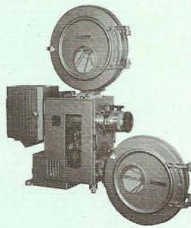
T60-HALOGEN 35mm PORTABLE SOUND PROJECTOR
