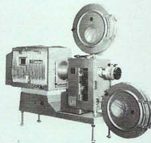
T-60X 35mm PROJECTOR WITH XENON LAMPHOUSE
